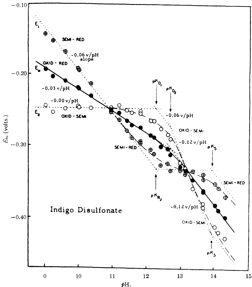
Fig. 4.—Oxidation-reduction potentials E_b of the component systems of indigo disulfonate at various pH .
