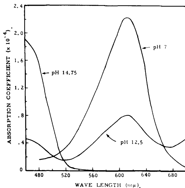
Fig. 1.—Shift of the absorption band of indigo disulfonate oxidant with pH change.
